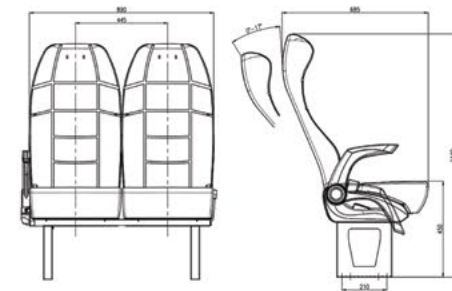
2D plain dimensions of the Seat
